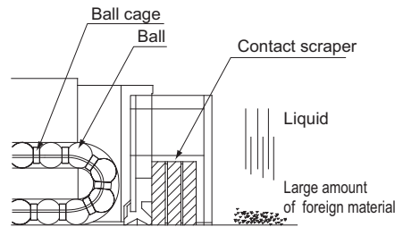
Structural Drawing
