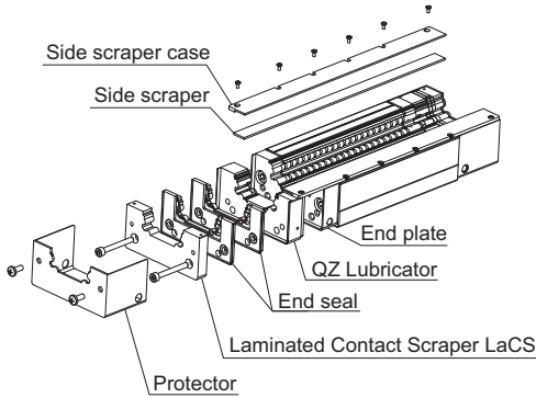
Outline view (Ex: in case of QZTTHYY type)
