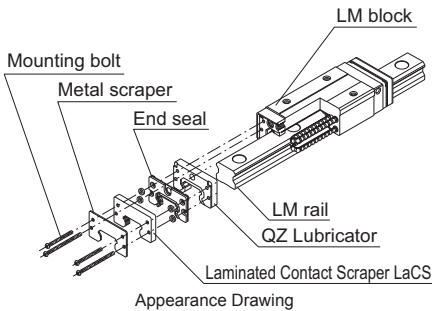
Appearance Drawing
