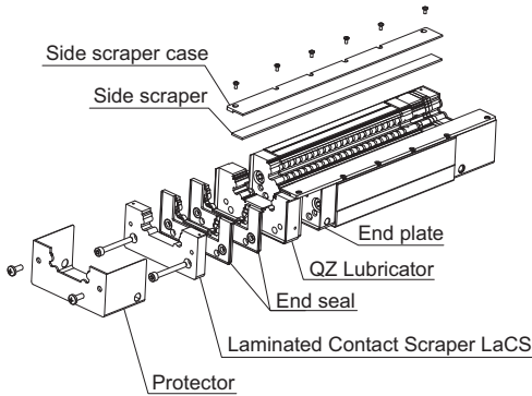
Outline view (Ex: in case of QZTTHHYY type)
