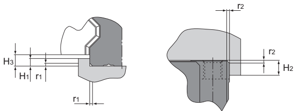
Shoulder for the LM Rail
